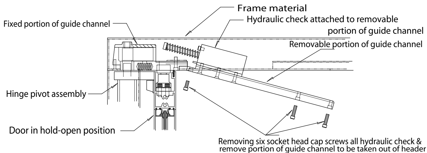
Partial elevation detail "B" showing check and removable portion of guide channel being removed from header while door is in hold-open position
