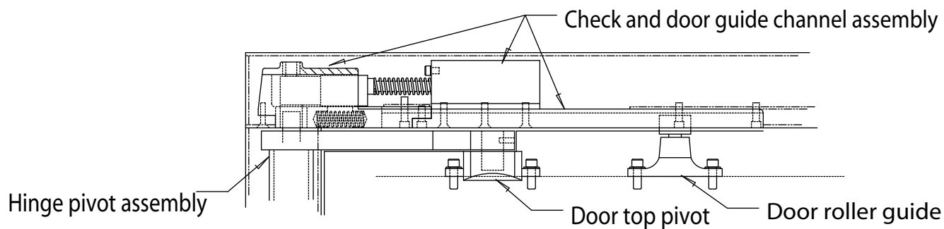
Partial elevation detail "A" showing check and guide channel assembly along with door in the closed position (face of door and frame omitted for clarity of hardware)
