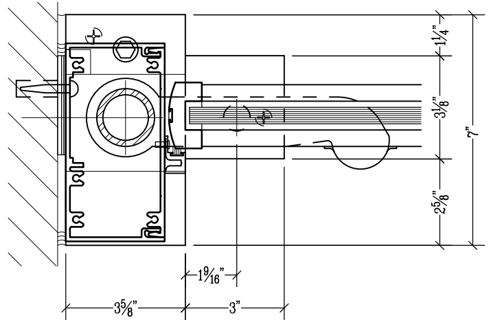
FLOORBOX WITH STANDARD HOLD-OPEN BOLT STRIKE (NO THRESHOLD)
