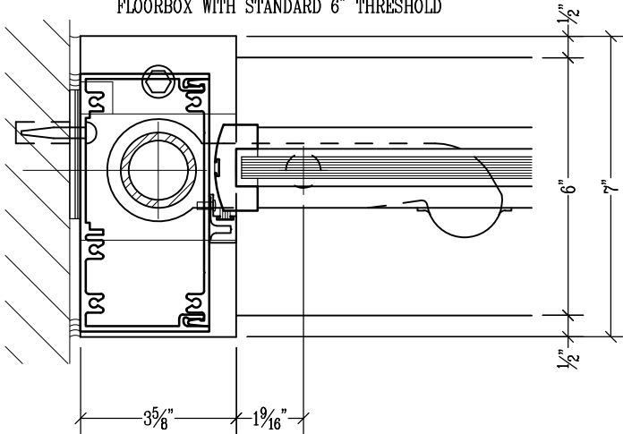
FLOORBOX WITH STANDARD 6" THRESHOLD
